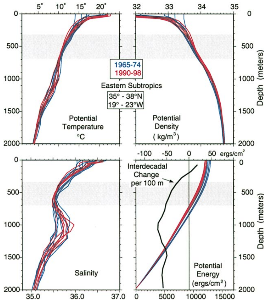
FIG. 11. Same as Fig. 10 but for the box labeled F in Fig. 8. Blue curves reflect low transport index years, red curves are high transport index years. Gray shading gives the depth range of the main thermocline. The black curve in the lower right panel is the PEA change between time frames per 100-m interval; its scale is on the top axis of that panel.
