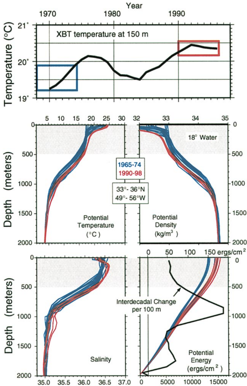
FIG. 10. Observed properties from the EDW formation region, labeled box B in Fig. 8. The top panel is a time series of temperature at 150 m from XBT measurements in the geographic area 34°–37°N, 50°–54°W (as in Molinari et al. 1997, but updated for this region by R. Molinari 2000, personal communication) Red and blue boxes mark the years of high and low transport extremes. The remaining panels are vertical profiles of potential temperature, density, salinity, and potential energy in the area 33°–36°N, 49°–56°W (the EDW formation region labeled box B in Fig. 8) at the extreme phases of the transport index: 1965–74 (blue curves) and 1990–98 (red curves). The curves represent the isopycnally averaged profiles in each 1° grid square within that geographic area for each time period. No additional smoothing has been performed. The gray shaded band in each panel depicts the depth range of the EDW. The black curve in the lower right panel (PEA profiles) reflects the magnitude of change between the two time periods for each 100-m depth increment; the scale is on top axis.
